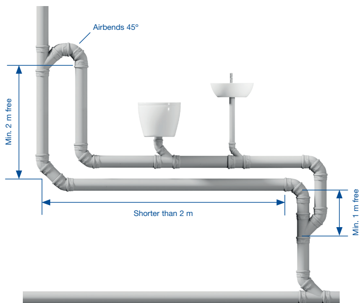
Fig. 14: Downpipe offset < 2 m, with bypass pipe and piping areas without connection points.
