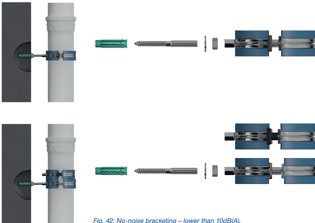
Fig. 42: No-noise bracketing – lower than 10dB(A).
