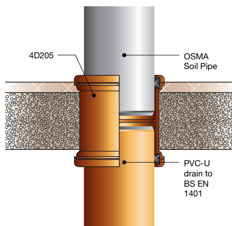
Figure 10: PVC-U drain spigot (via 4D205)
