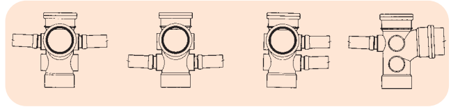
Figure 20: Permitted connections
