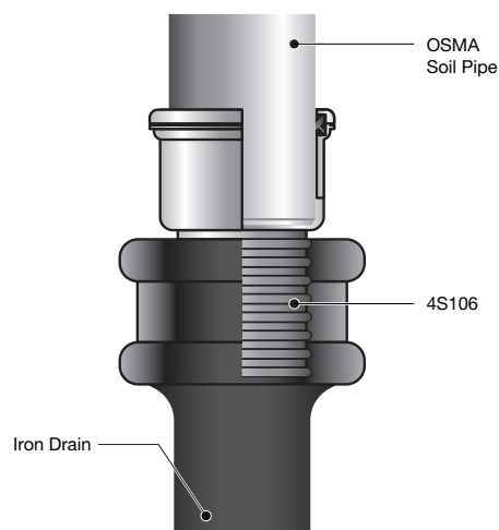
Figure 49: Cast iron drain socket
