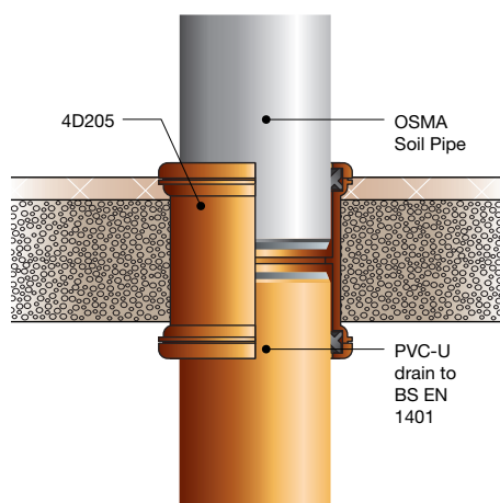
Figure 47: PVC-U drain spigot (via 4D205)
