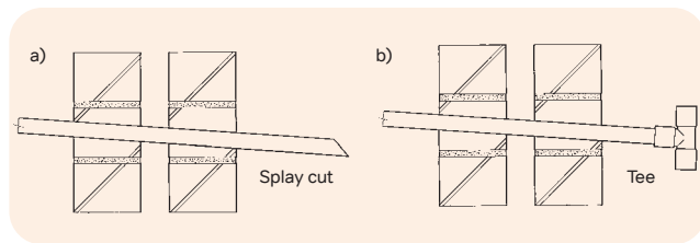
Figure 70: Terminating overflow pipe
