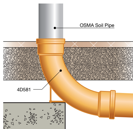
Figure 9: PVC-U drain socket (via 4D581)
