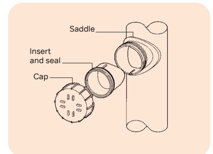
Figure 51: Access Saddle
