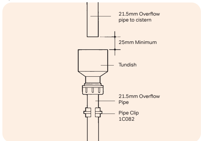
Figure 72: Tundish connection to 21.5mm Push-Fit Overflow Pipe
