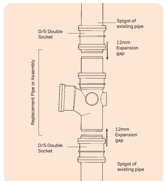
Figure 76: Incorporating a fitting
