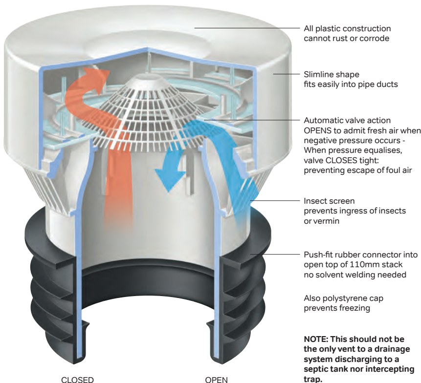
Figure 32: Valve operation
