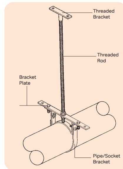
Figure 45: Suspended Bracketing (intermediate pipe support)
