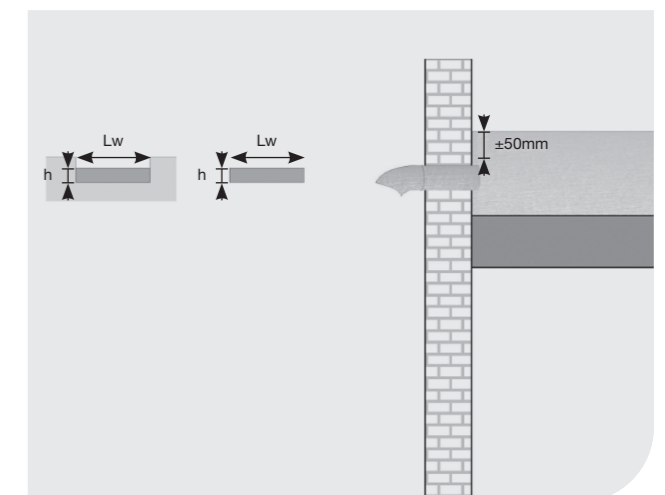
Figure 29: Calculation rectangular emergency overflow
