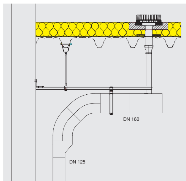
Figure 24: Downpipe reduced
