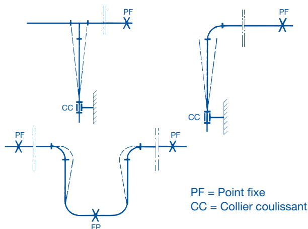
Figure 3 Points fixes et colliers
