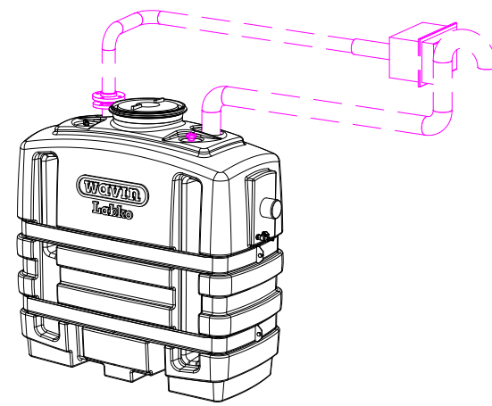
EuroREK NS2 SL (EN1825) grease separator (indoor installation, on the floor) Max. flow rate 2 l/s
