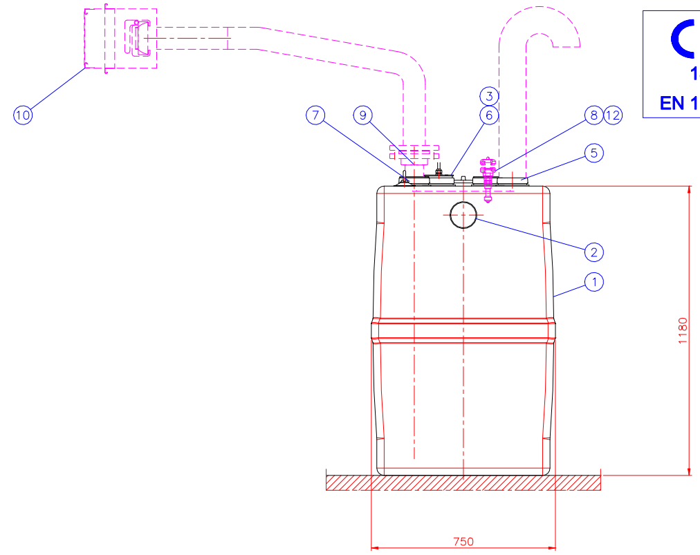
Indoor installation model (On the floor)
