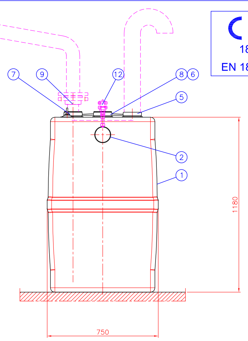
Indoor installation model (On the floor)
