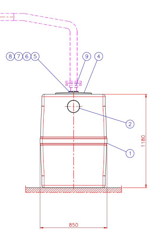
Indoor installation model (On the floor)
