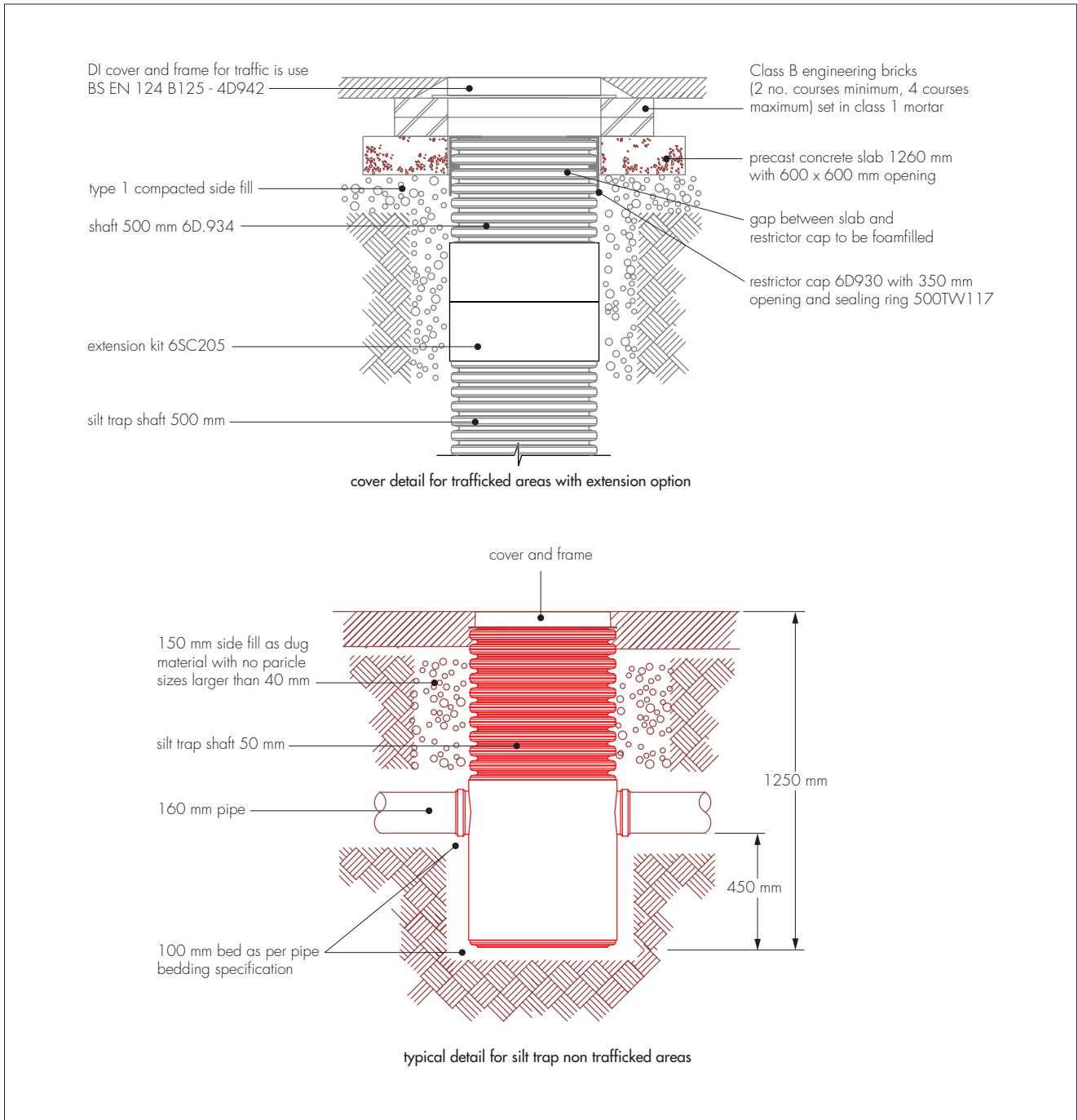
Figure 5 Typical silt trap
