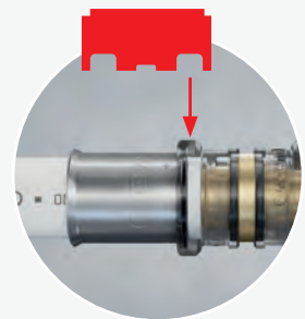
TH-B-Konturen 25–40 mm
