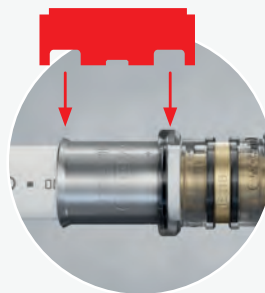
TH-B-Konturen 16–20 mm
