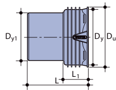
X-Stream pipe - smooth PVC socket
