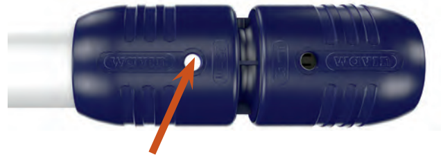
Figure 8: The observation window in the PPSU cap can be used to check that the pipe is inserted to the stop.
