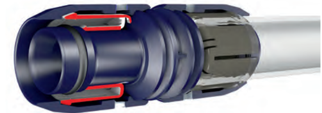
Figure 9: The smartFiX push-fit fitting.
