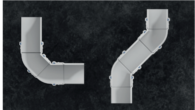
Fig. 20: Changes of direction with 45° bend.
