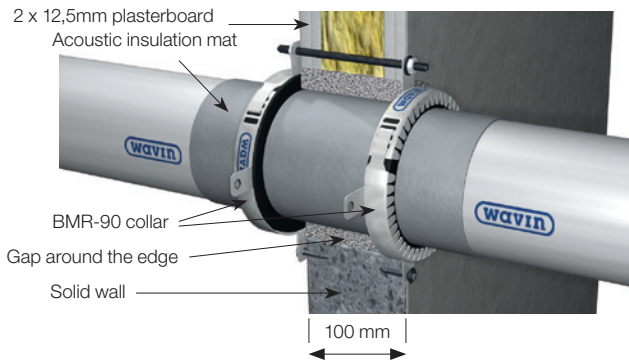
Fig. 51: Straight installation without sleeve / socket.
