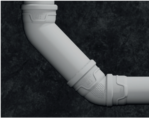
Fig. 34: Extended 45° bend.
