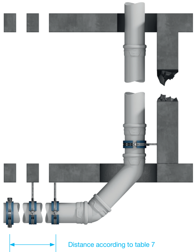
Figure. 26: Example horizontal and vertical installation.
