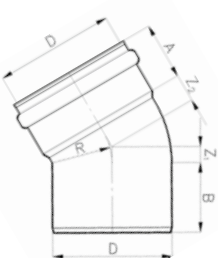
Solidwall PVC SN12 - Koleno 30°
