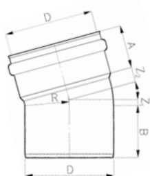
Solidwall PVC SN12 - Koleno 15°
